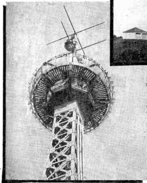
WENA (Detroit) FM tower atop the Penobscot Building. Licensed to the Evening News Association (WWJ).
